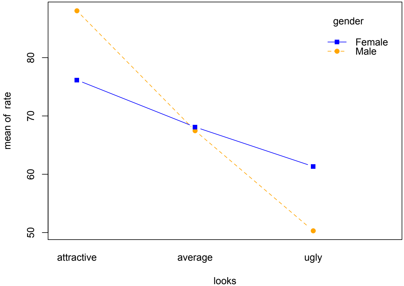
Interaction plot: looks by gender
